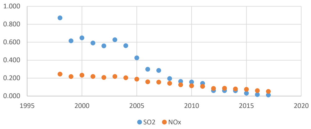
Figure 3: NYS Statewide SO 2 and NO x Rates (lbs/mmBtu)
