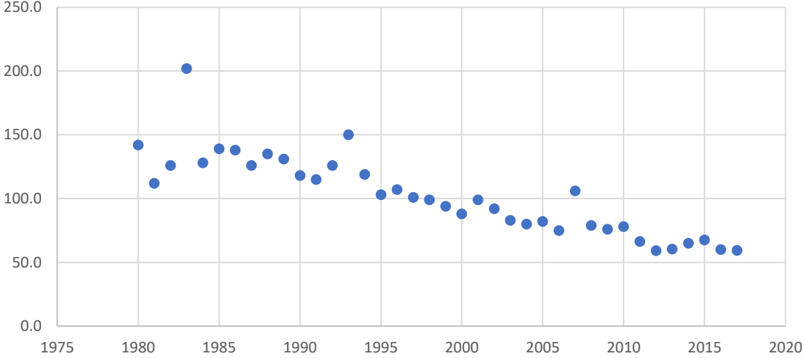
NYS Maximum Annual Ambient NO2 Max 98th Percentile
