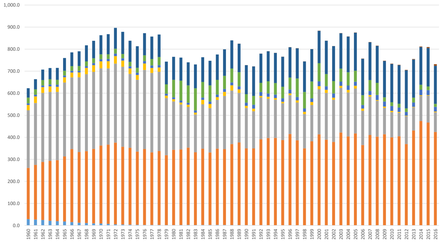
NYS Net Residential Energy Consumption (TBtu)
