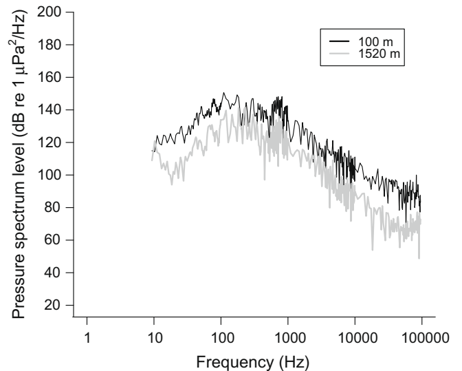
Fig. 4. Power spectral density of three seconds of pile-driving noise at 100 m and 1520 m distance. Recordings of pile-driving noise were made with Brüel and Kjaer 8104 and 8105 hydrophones. The data was over the frequency range 10 Hz to 96 kHz without correcting for sensitivity variations above 10 kHz.
