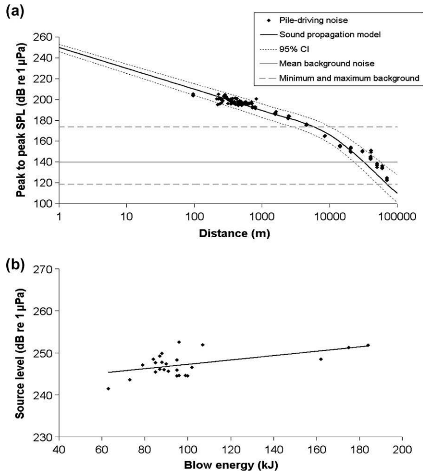
Fig. 5. (a) Broadband peak to peak sound pressure levels of pile-driving in relation to distance from the noise source and the best-fit sound propagation model. Peak to peak background noise levels are shown for comparison only. (b) Relationship between estimated peak to peak source level of pile-driving noise and blow energy of piling hammer with least-squares regression line.
