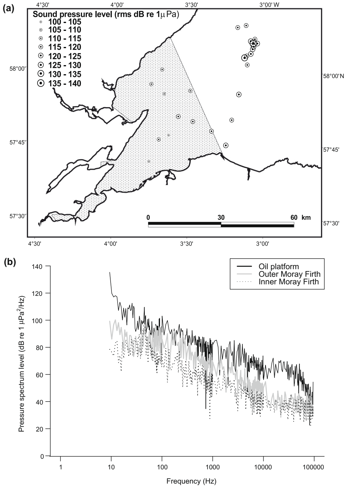
Fig. 2. (a) Location and sound pressure level (root mean square) of background noise measurements, the Marine Protected Area is shaded, (b) Power spectral density of three seconds of background noise measured in the vicinity (800 m distance) of the operating oil platform, at the outer boundary of the Marine Protected Area (outer Moray Firth) and within the Marine Protected Area (inner Moray Firth). Recordings of background noise were made with a Brüel and Kjaer 8106 hydrophone, sampling at 300 kHz and 24 bit depth. The data was summed over the frequency range from 10 Hz to 120 kHz without correcting for the high frequency roll off above 80 kHz.
