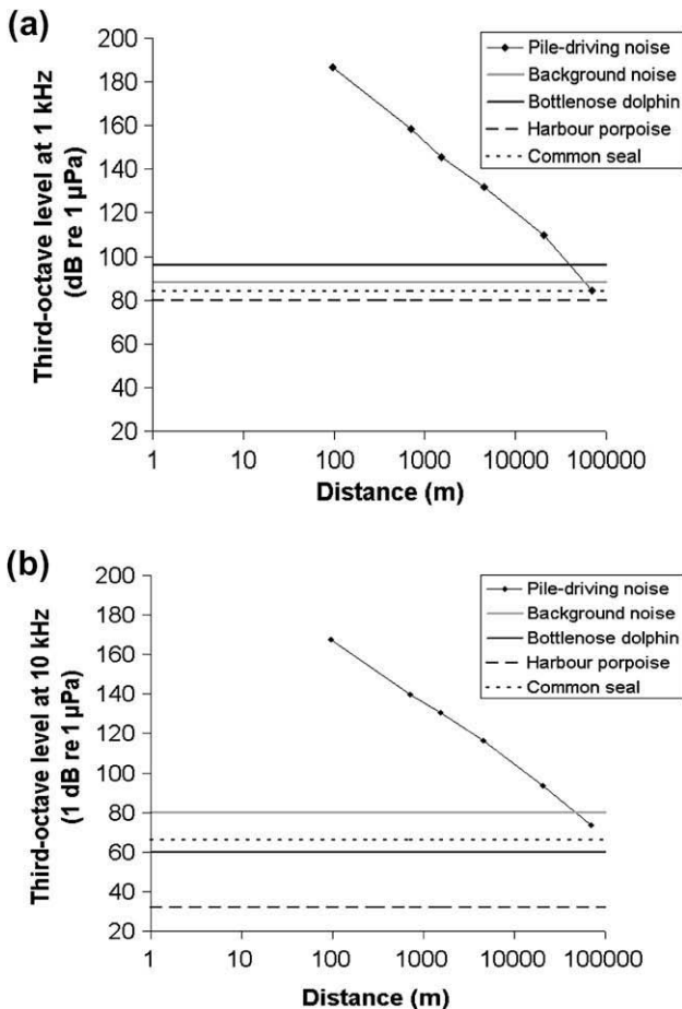
Fig. 6. Third-octave band sound levels for pile-driving at 96 m to 70 km range, the mean third-octave band background noise levels and hearing thresholds for bottlenose dolphins, harbour porpoises and common seals at (a) 1 kHz and (b) 10 kHz.
