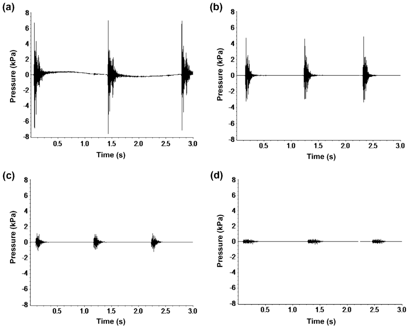
Fig. 3. Three-second time histories of underwater pile-driving noise at a distance of (a) 100 m, (b) 710 m, (c) 1520 m, (d) 4550 m.
